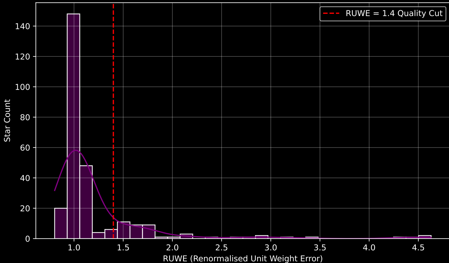
GALAH DR4 Field [633] RUWE Distribution (n= 271)
