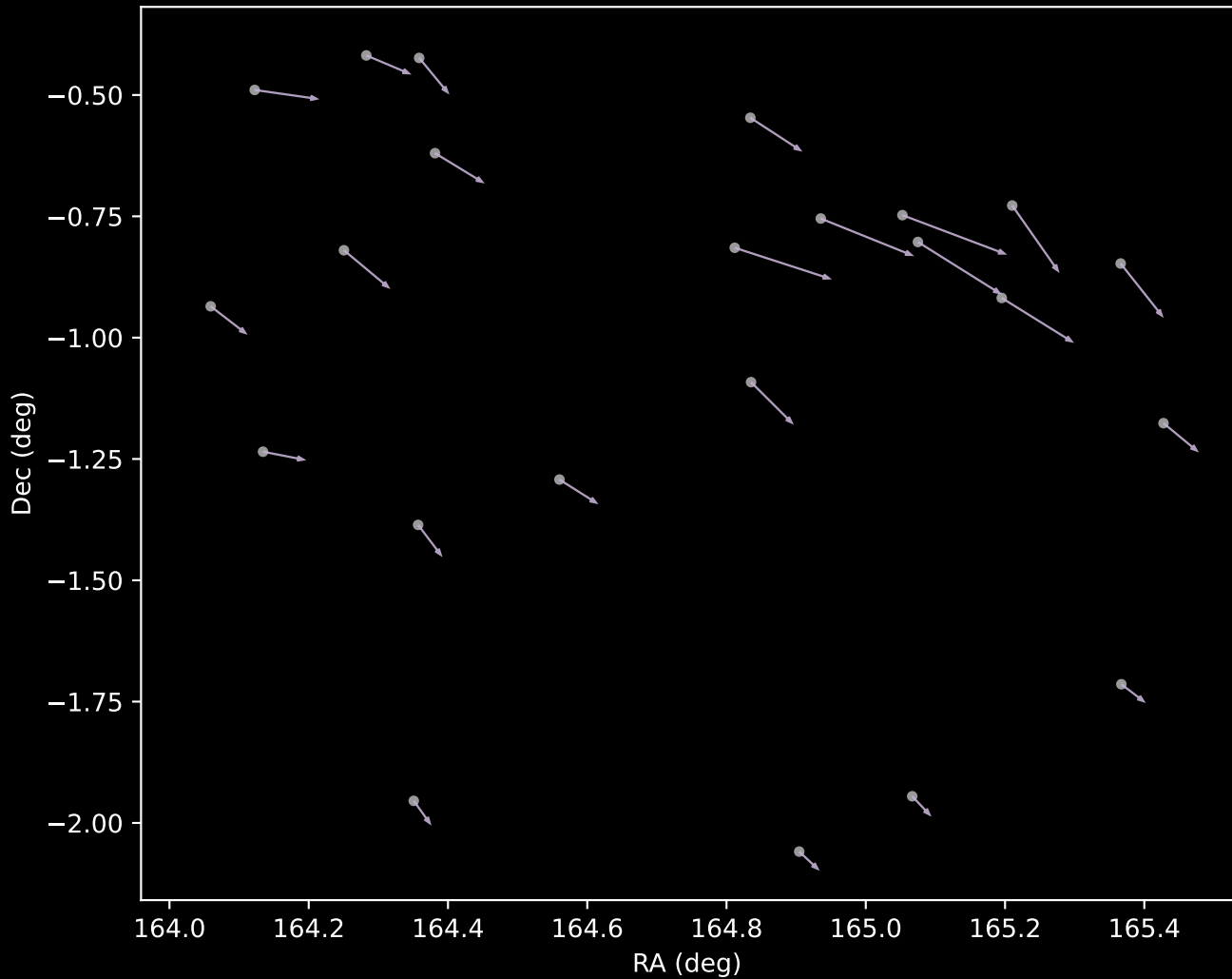
GALAH DR4 Cluster 9 Proper Motion Vectors (n=23)
