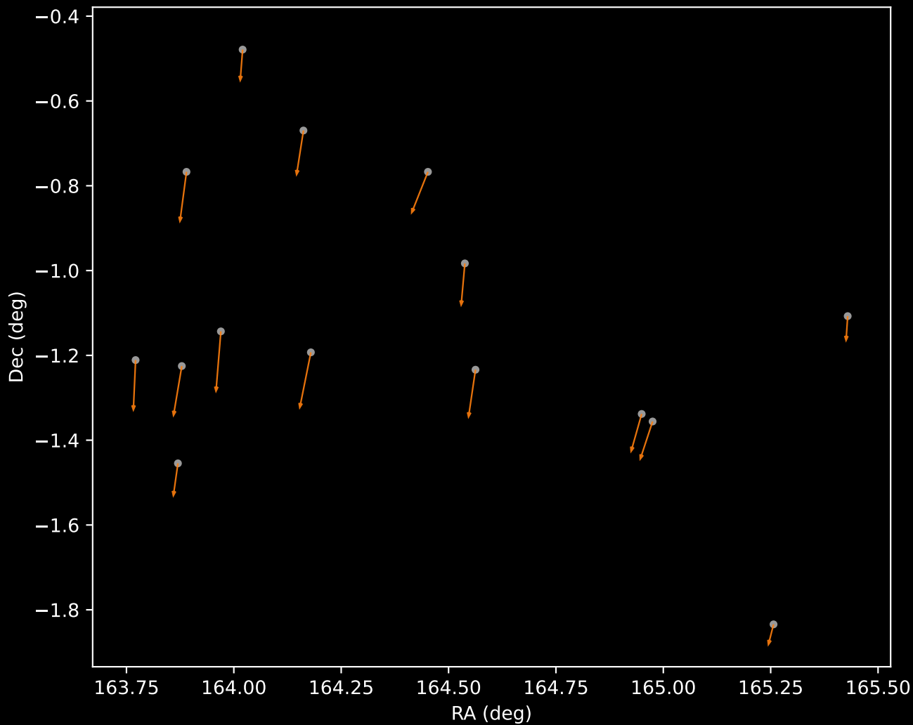
GALAH DR4 Cluster 2 Proper Motion Vectors (n=15)
