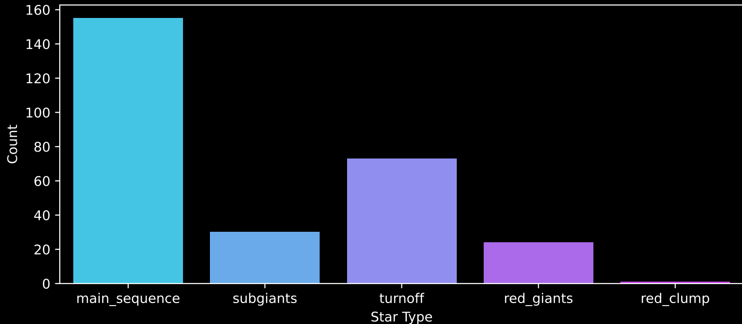
GALAH DR4 Field: [633] Count plot of Star Type
