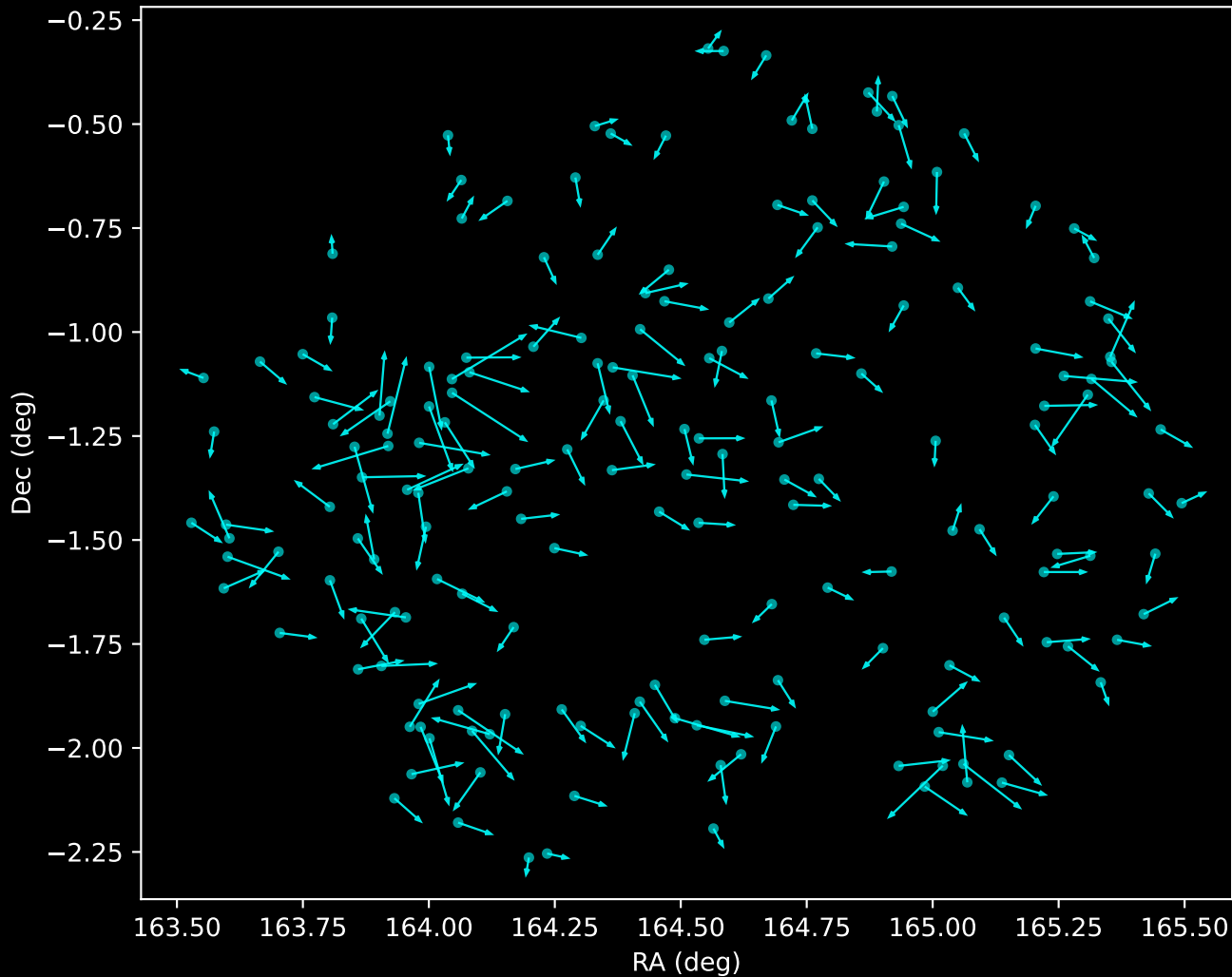
GALAH DR4 Noise Stream Proper Motion Vectors (n=182)
