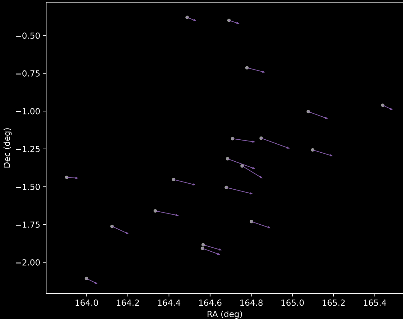
GALAH DR4 Cluster 8 Proper Motion Vectors (n=19)
